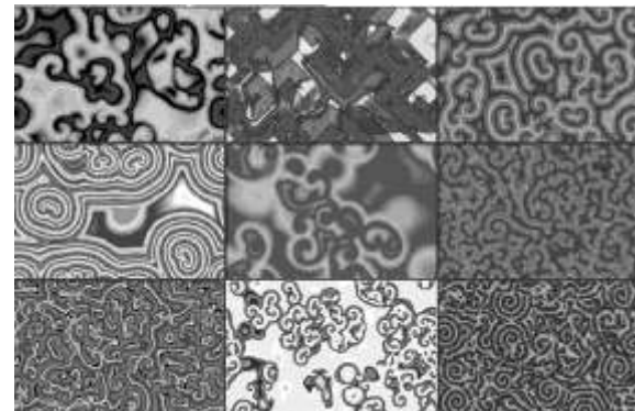
Figure 3: Gnarly Two-Dimensional Cellular Automata
